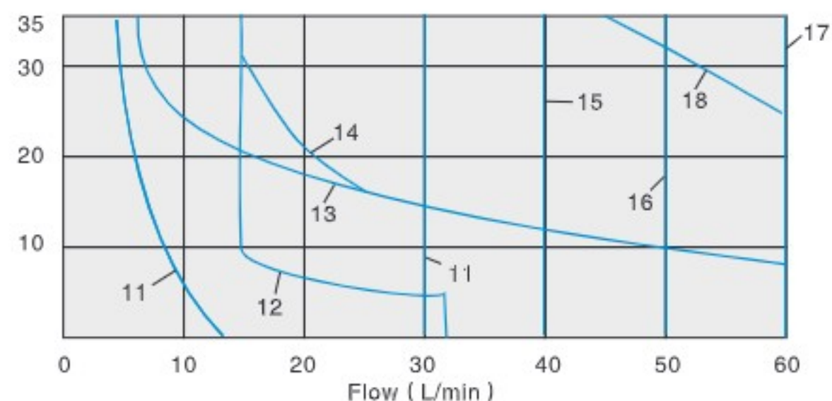
Working pressure(MPa)
